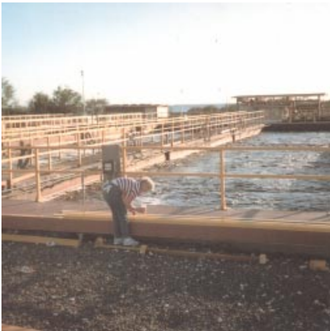
Above: Lightweight, corrosion resistant 24" fiberglass I-beams span 45' to bridge clarifiers at the Las Rusias, Texas Waste Water Treatment Plant. Left: 2500 feet of handrail was installed at the Fort Kamehameha Wastewater Treatment Facility, Pearl Harbor Naval Base in Hawaii.
